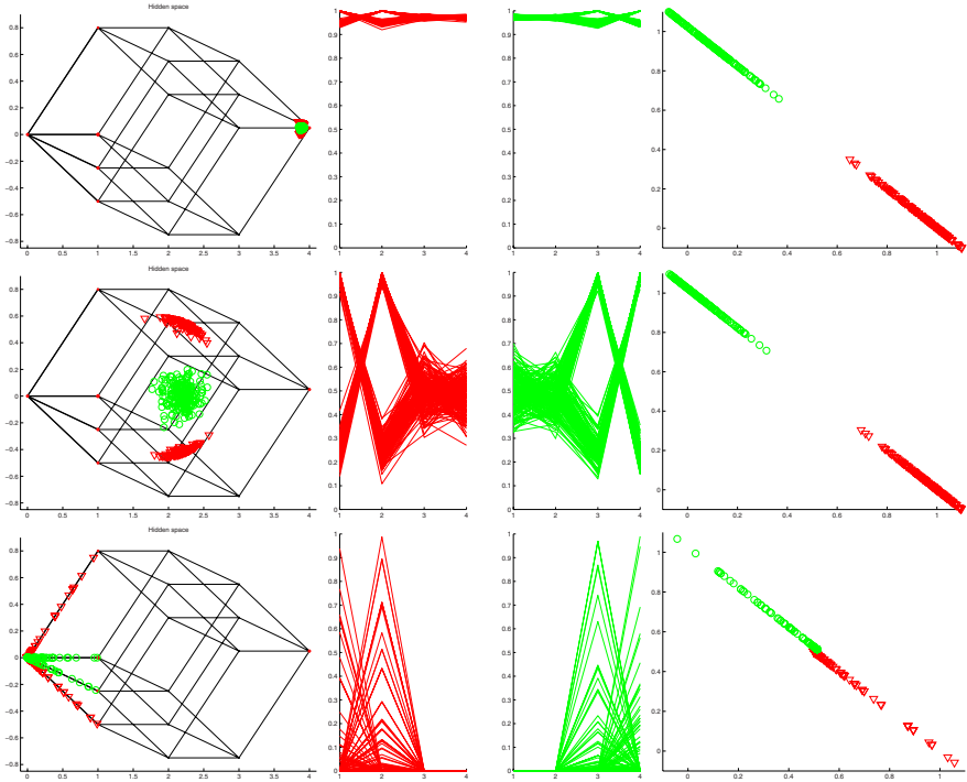
Fig. 1. RBF solution of the noisy XOR problem, using 4 Gaussians; for dispersion \sigma = 7 the map is clustered in the (1,1,1) corner of the hypercube (top row) for \sigma = 1 optimum separation is achieved (middle row), and for \sigma = 1/7 all activities are very small (bottom row). See text for description.
