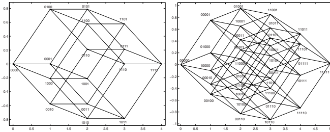
Fig. 1. Lattices corresponding to the vertices of 4 and 5-dimensional hypercubes, obtained by linear projection of their vertices.
