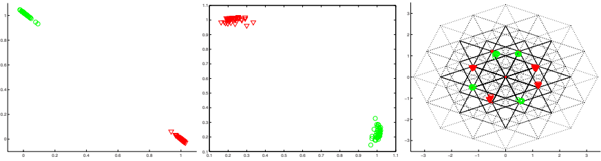
Fig. 4. 3 bit fuzzy parity problem solved with RBF network with 8 Gaussian nodes. Left: outputs show perfect separation; middle: reduced internal space shows perfect clustering; right: lattice projection show clusters around coordinate axes.
