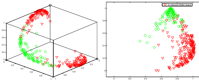
Fig. 3. Left: 3 hidden Gaussian nodes trained on the XOR data; right: reduced representation.
