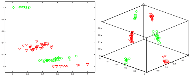
Fig. 5. 3 bit fuzzy parity problem solved with RBF network with 2 and 3 Gaussian nodes. Although errors are at the base rate level images in the internal space are well clustered.
