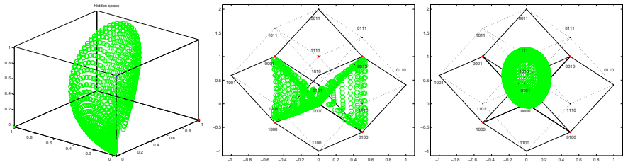
Fig. 2. A mesh spanning all possible input values mapped using RBF network with 3 hidden nodes trained on the Iris data (left) and with 4 nodes trained on the noisy XOR data with \sigma = 0.25 and \sigma = 1.5 shows the admissible subspace of hidden node activations.
